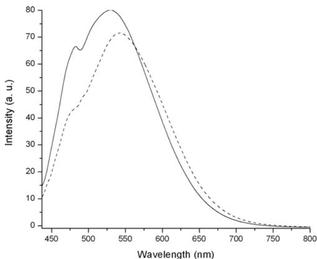
Figure 1. Fluorescent spectra of 1 (solid line) and 2 (dashed line) in 1,1,2-trichloroethane (conc. 1.3 \cdot 10^{-5} M, excitation wavelength = 420 nm).
