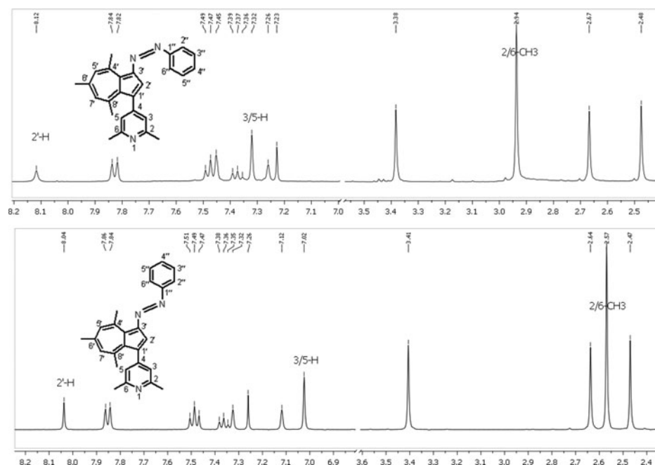
Figure 7. 1 H-NMR spectra of 2 in CDCl 3 , before (down) and after UV irradiation (top). The NMR scale is truncated for better comparison.
