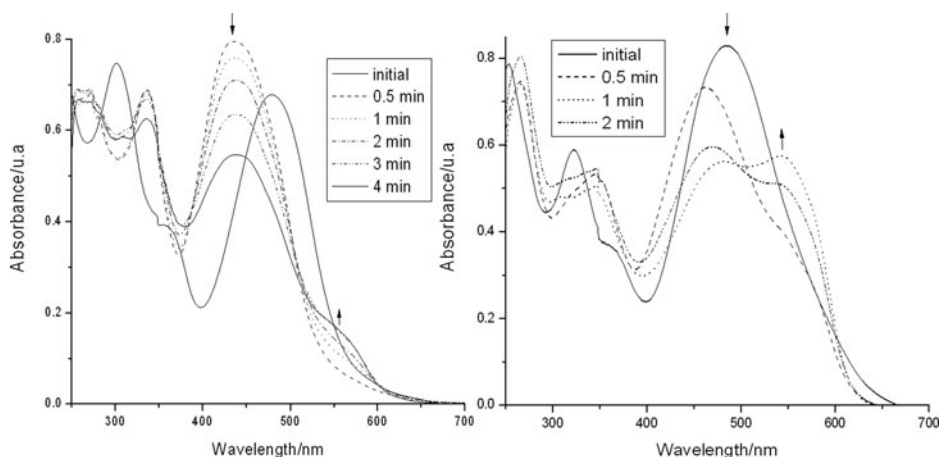
Figure 6. Absorption spectra of compounds 3 and 4 in \text{CHCl}_3 solutions under 254 nm irradiation. The exposure time is shown in the inset legends.
