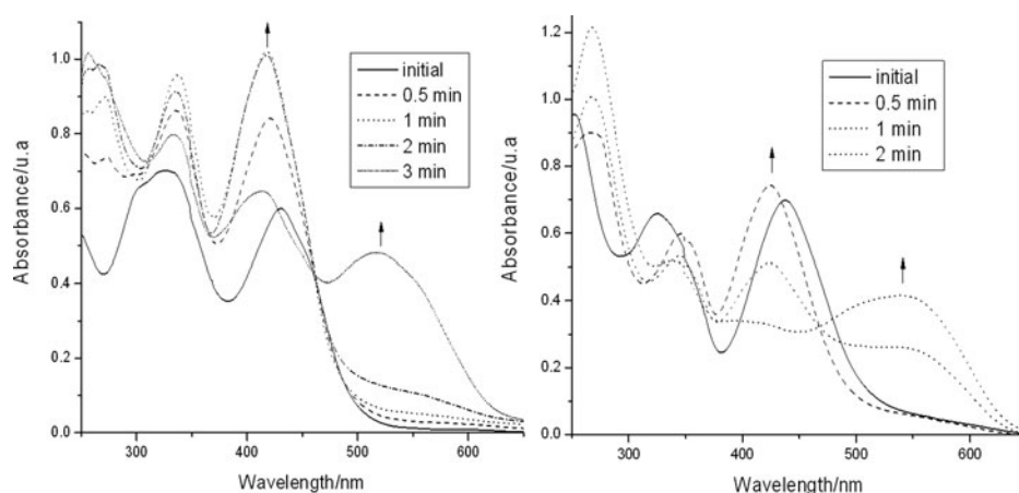
Figure 5. Absorption spectra of compounds 1 and 2 in CHCl 3 solutions under 254 nm irradiation. The exposure time is shown in the inset legends.
