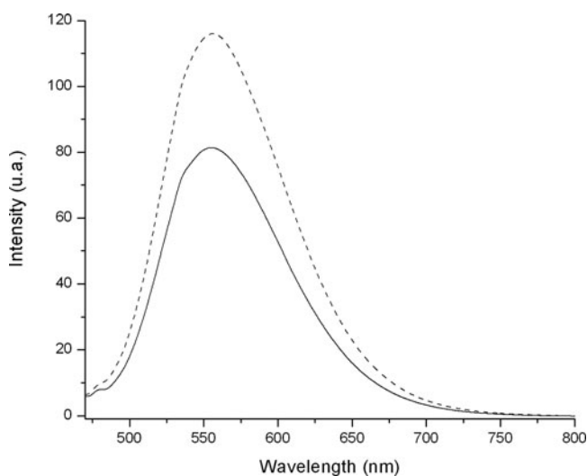
Figure 2. Fluorescent spectra of 3 (solid line) and 4 (dashed line) in 1,1,2-trichloroethane (conc. 0.6 \cdot 10^{-5} M, excitation wavelength = 460 nm).
