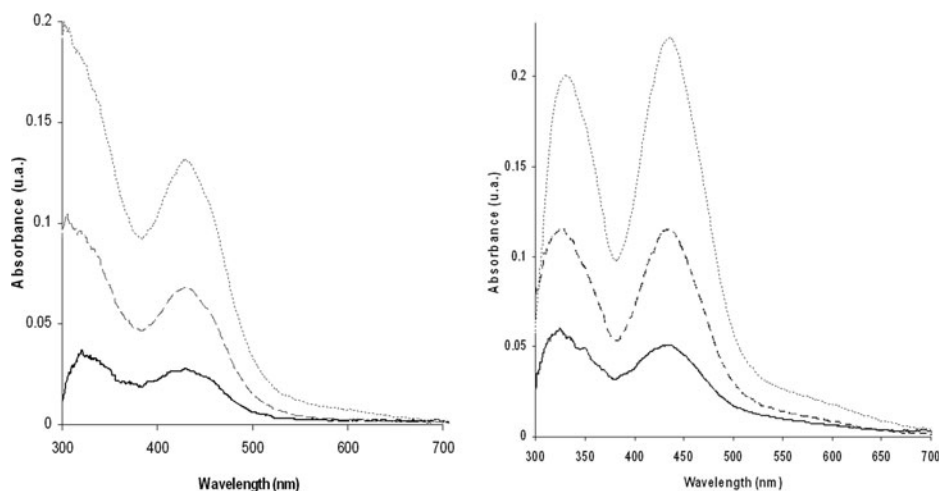
Figure 4. UV-Vis spectra of PMMA thin films containing compound 1 (left side) and compound 2 (right side) of different loadings: 2% (solid line), 5% (dashed line) and 10% (dotted line).
